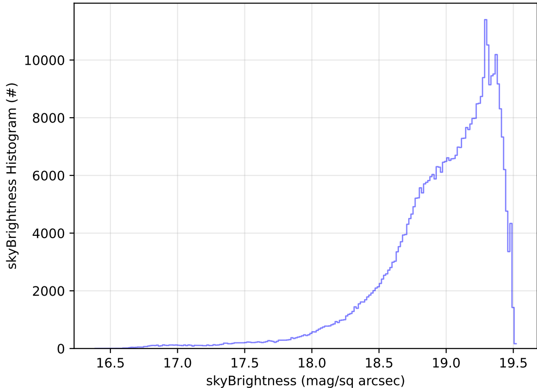
ddf_acor_sf30_lsf40_lsr20_v3.4_10yrs All sky z band: skyBrightness Histogram
