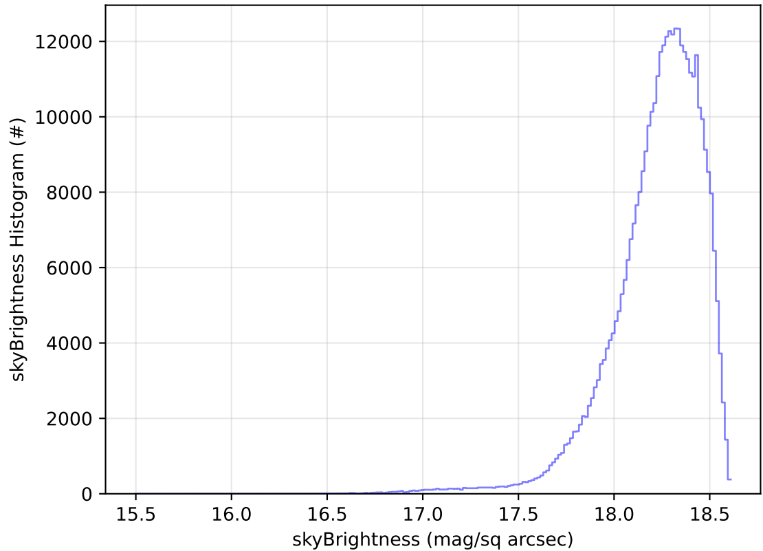
ddf_acor_sf30_lsf40_lsr20_v3.4_10yrs All sky y band: skyBrightness Histogram
