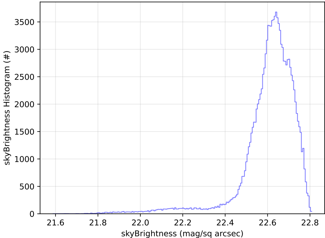
ddf_acor_sf30_lsf40_lsr20_v3.4_10yrs All sky u band: skyBrightness Histogram
