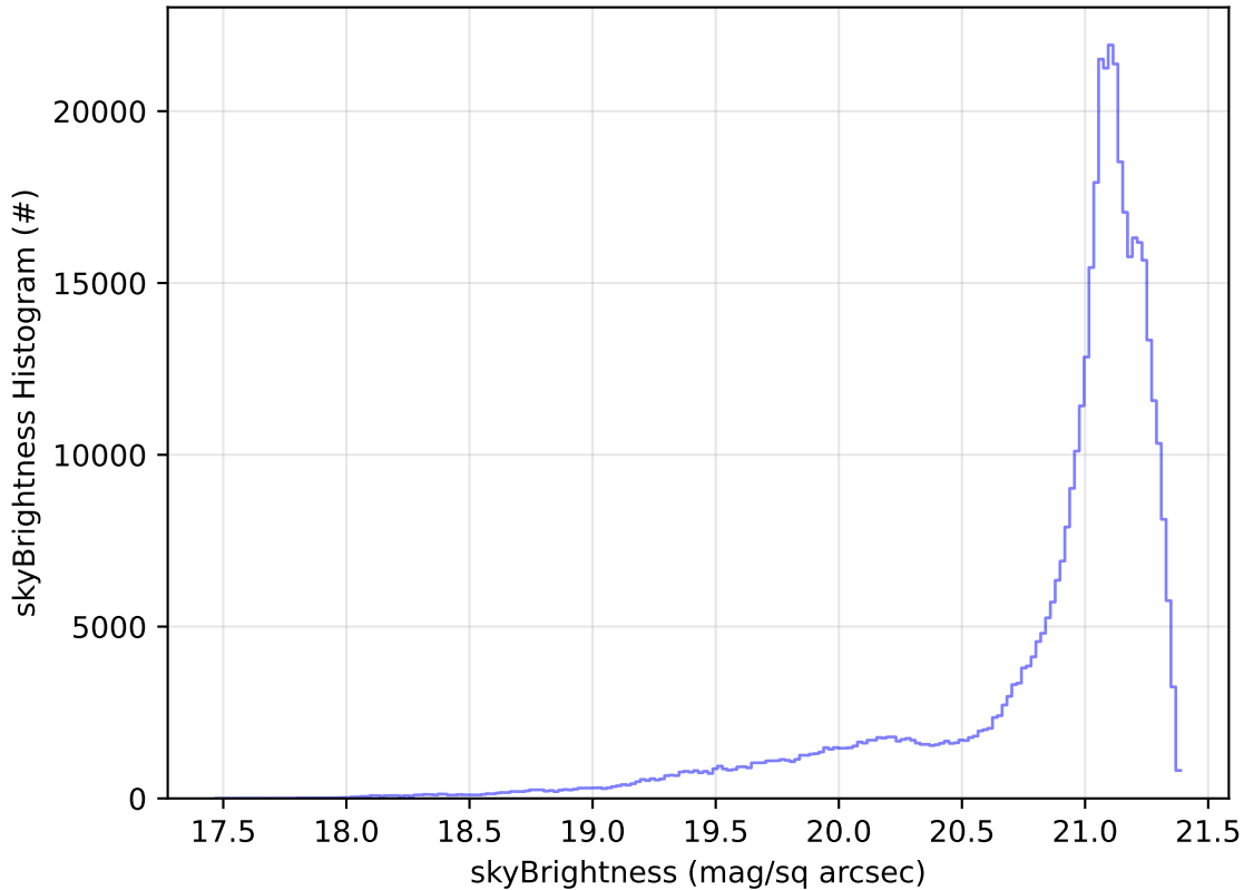
ddf_acor_sf30_lsf40_lsr20_v3.4_10yrs All sky r band: skyBrightness Histogram
