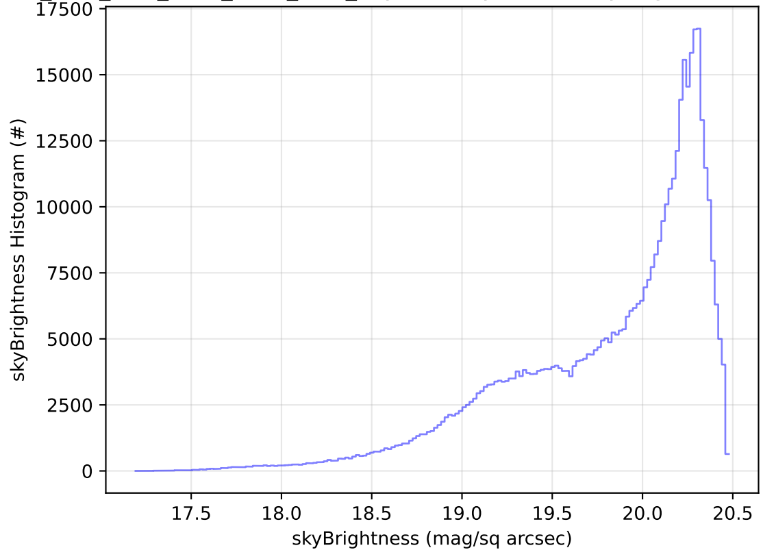
ddf_acor_sf30_lsf40_lsr20_v3.4_10yrs All sky i band: skyBrightness Histogram
