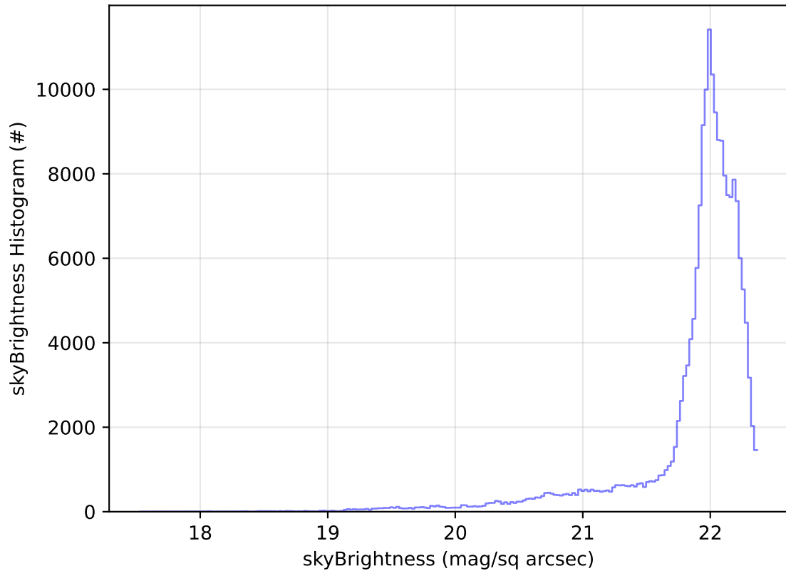
ddf_acor_sf30_lsf40_lsr20_v3.4_10yrs All sky g band: skyBrightness Histogram
