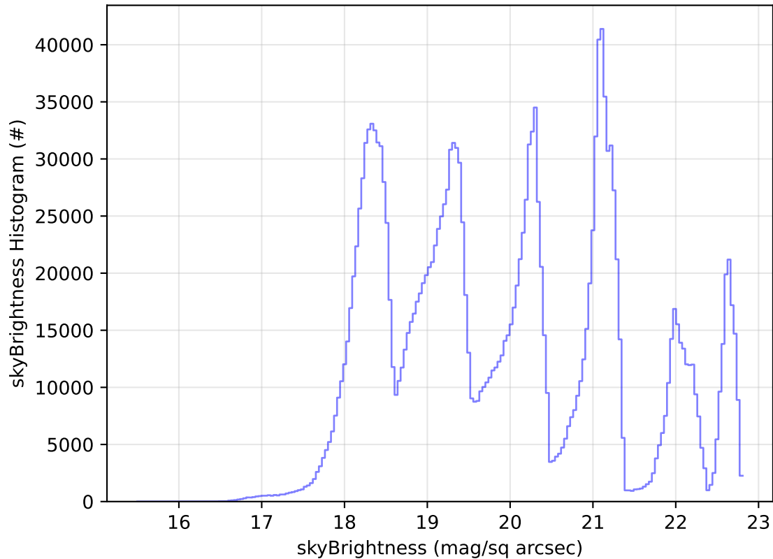
ddf_acor_sf30_lsf40_lsr20_v3.4_10yrs All sky all bands: skyBrightness Histogram
