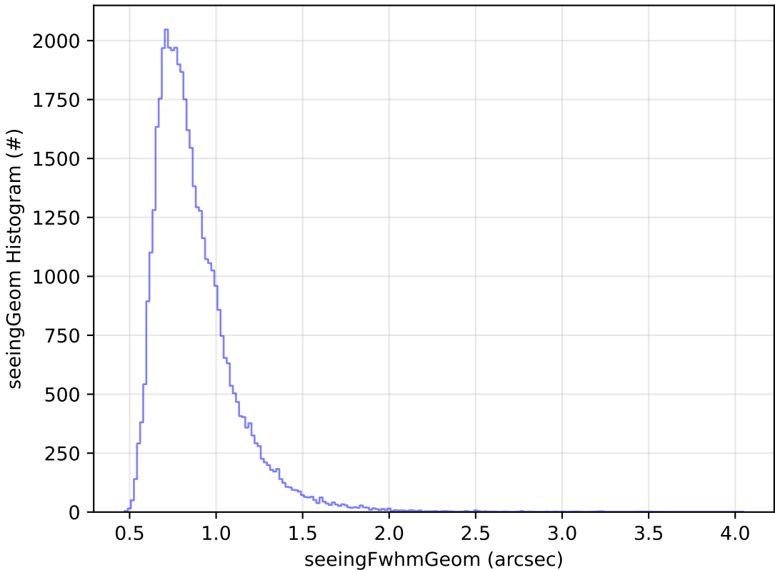
ddf_acor_sf30_lsf40_lsr20_v3.4_10yrs Yr 1 z band: seeingGeom Histogram
