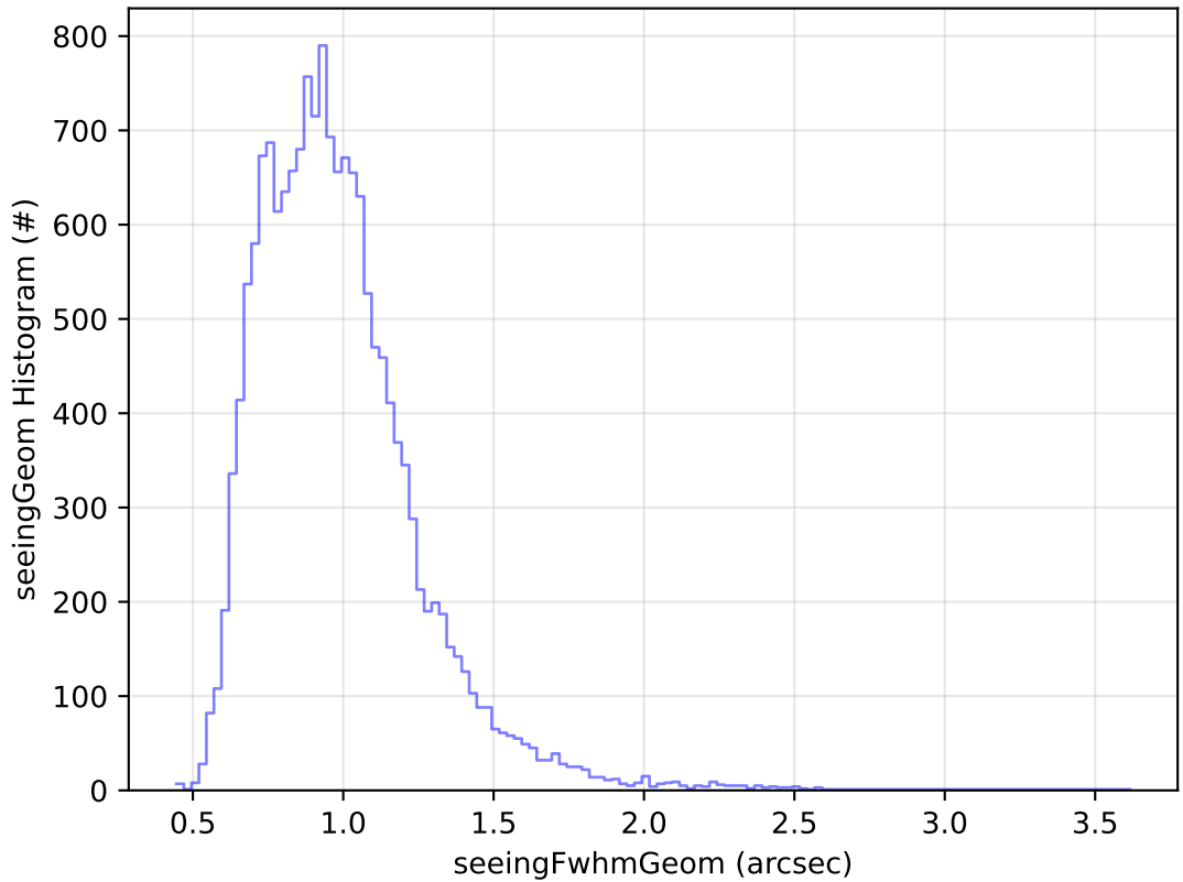
ddf_acor_sf30_Isf40_Isr20_v3.4_10yrs Yr 1 u band: seeingGeom Histogram
