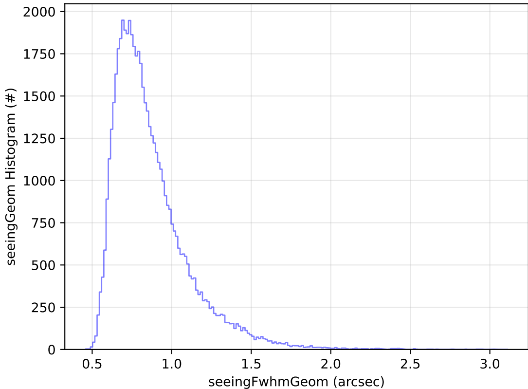
ddf_acor_sf30_lsf40_lsr20_v3.4_10yrs Yr 1 i band: seeingGeom Histogram
