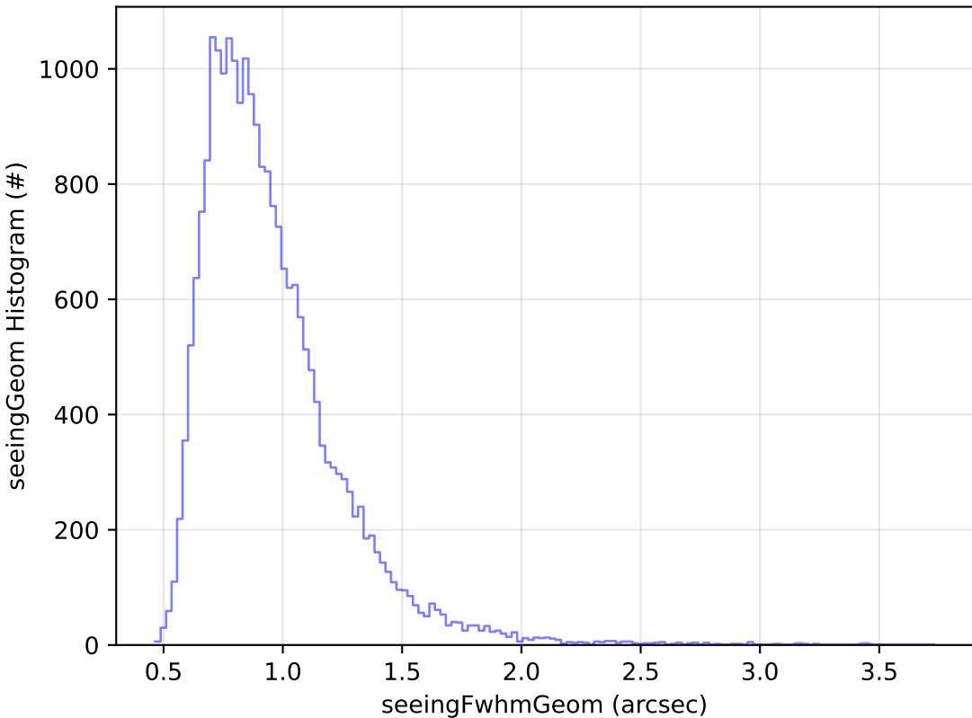
ddf_acor_sf30_lsf40_lsr20_v3.4_10yrs Yr 1 g band: seeingGeom Histogram
