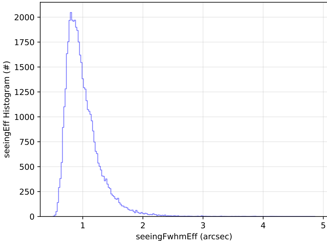
ddf_acor_sf30_lsf40_lsr20_v3.4_10yrs Yr 1 z band: seeingEff Histogram
