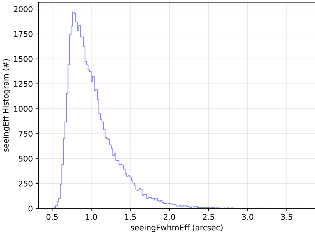
ddf_acor_sf30_lsf40_lsr20_v3.4_10yrs Yr 1 r band: seeingEff Histogram
