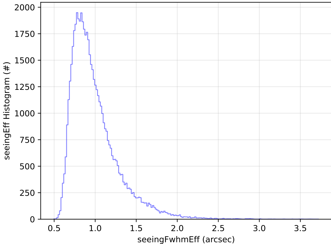
ddf_acor_sf30_lsf40_lsr20_v3.4_10yrs Yr 1 i band: seeingEff Histogram
