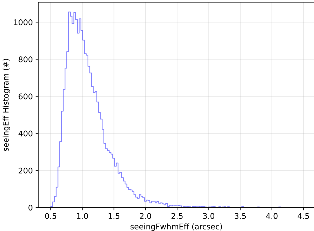
ddf_acor_sf30_lsf40_lsr20_v3.4_10yrs Yr 1 g band: seeingEff Histogram
