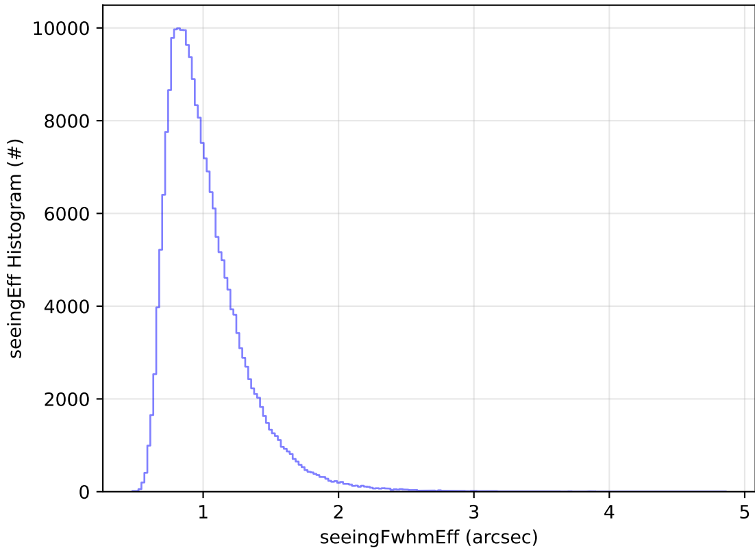
ddf_acor_sf30_Isf40_Isr20_v3.4_10yrs Yr 1 all bands: seeingEff Histogram
