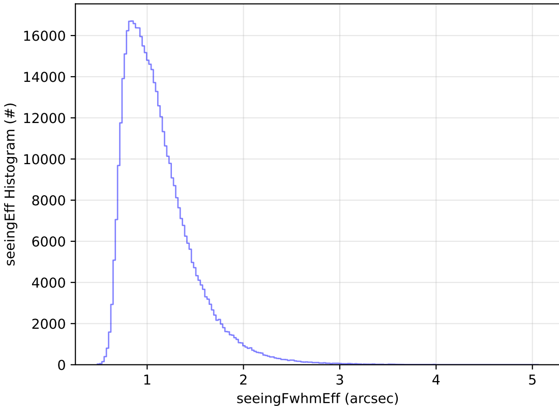
ddf_acor_sf30_lsf40_lsr20_v3.4_10yrs WFD r band: seeingEff Histogram
