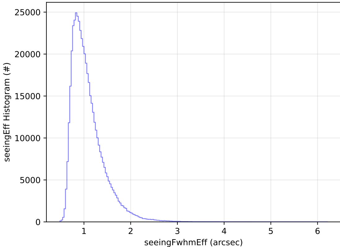
ddf_acor_sf30_lsf40_lsr20_v3.4_10yrs WFD i band: seeingEff Histogram
