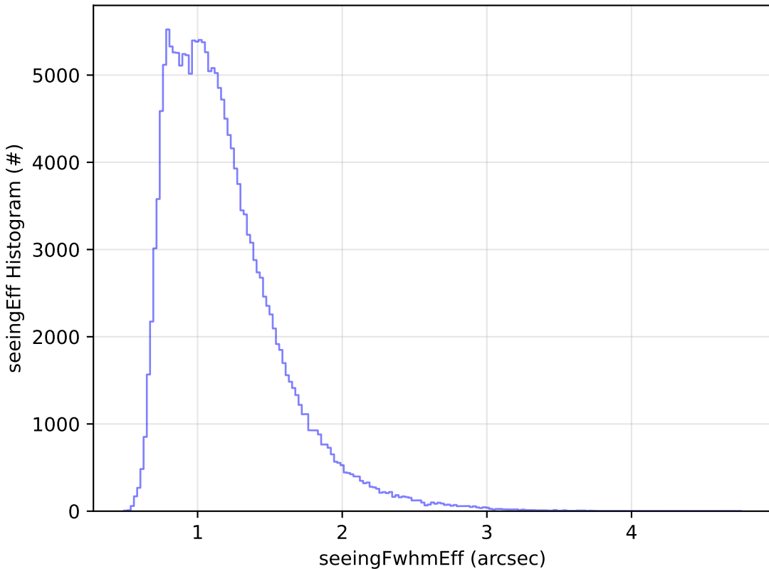
ddf_acor_sf30_lsf40_lsr20_v3.4_10yrs WFD g band: seeingEff Histogram
