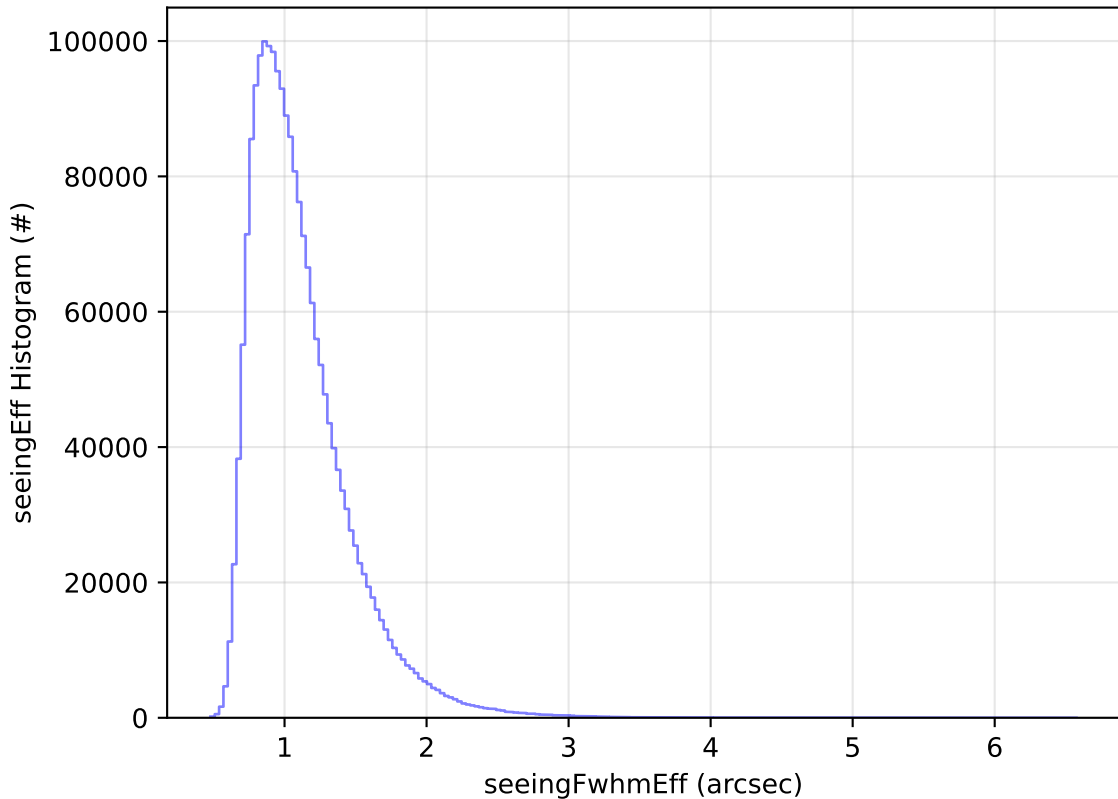
ddf_acor_sf30_lsf40_lsr20_v3.4_10yrs WFD all bands: seeingEff Histogram
