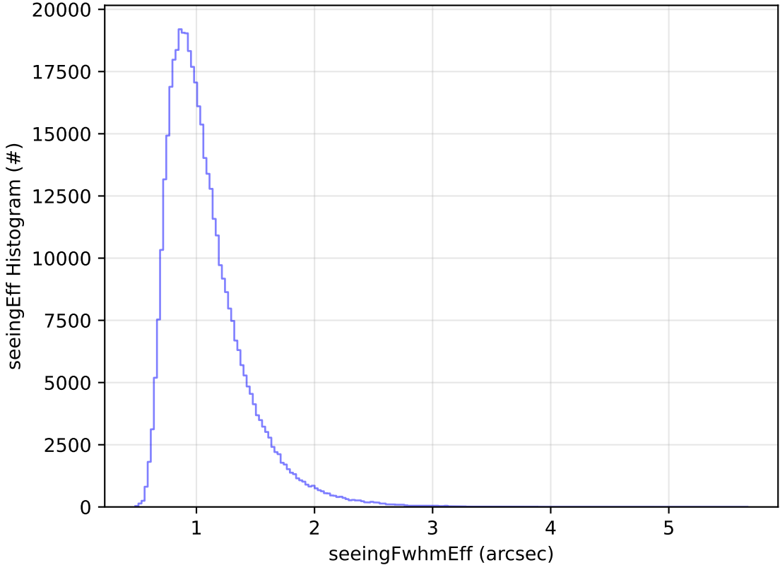
ddf_acor_sf30_Isf40_Isr20_v3.4_10yrs All sky z band: seeingEff Histogram
