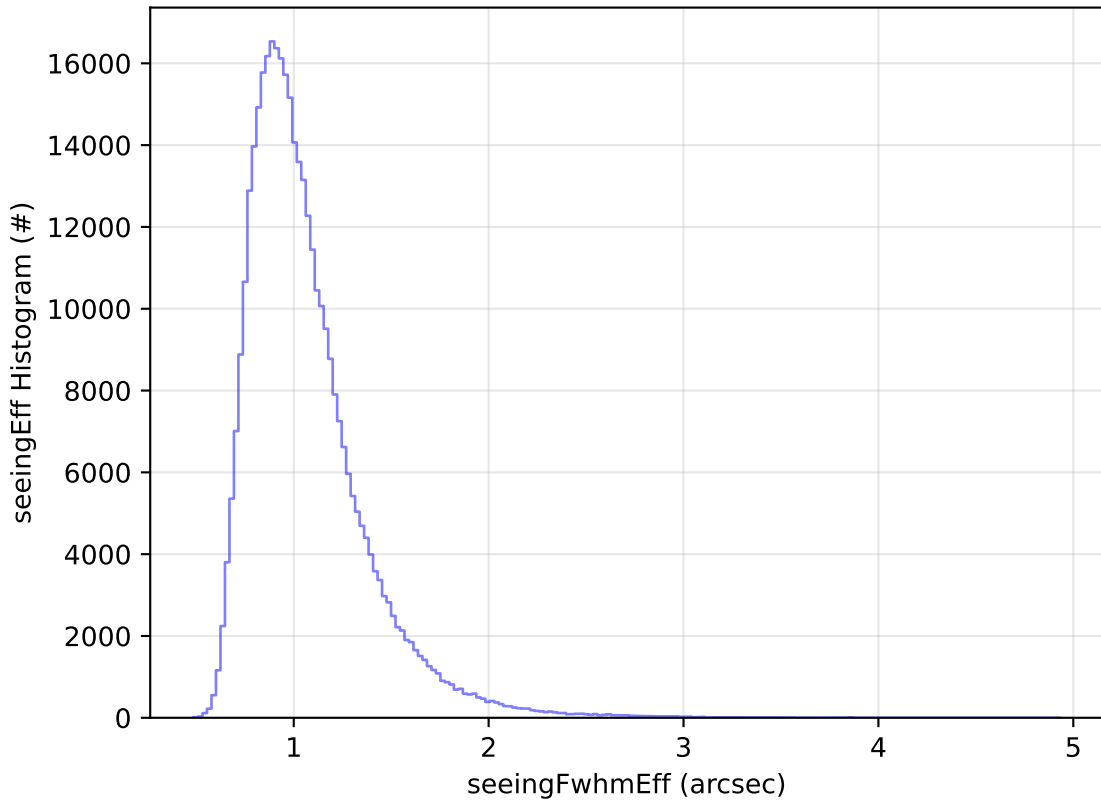
ddf_acor_sf30_lsf40_lsr20_v3.4_10yrs All sky y band: seeingEff Histogram
