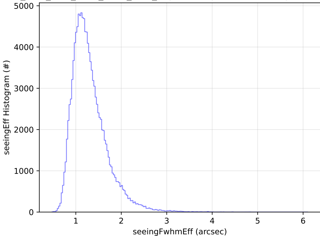
ddf_acor_sf30_ls40_lsr20_v3.4_10yrs All sky u band: seeingEff Histogram
