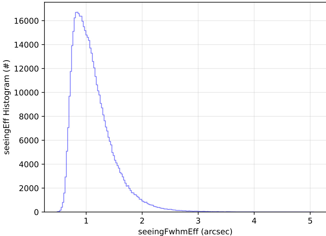
ddf_acor_sf30_Isf40_Isr20_v3.4_10yrs All sky r band: seeingEff Histogram
