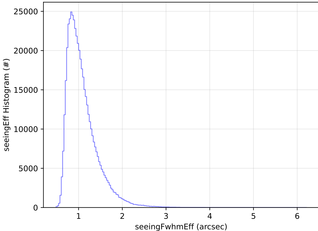
ddf_acor_sf30_lsf40_lsr20_v3.4_10yrs All sky i band: seeingEff Histogram
