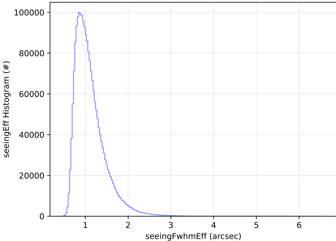
ddf_acor_sf30_lsf40_lsr20_v3.4_10yrs All sky all bands: seeingEff Histogram
