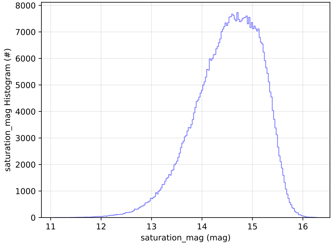
ddf_acor_sf30_lsf40_lsr20_v3.4_10yrs WFD r band: saturation_mag Histogram
