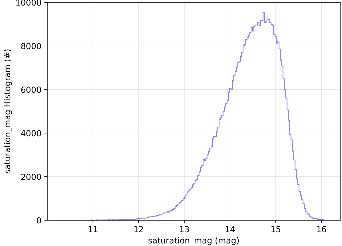
ddf_acor_sf30_lsf40_lsr20_v3.4_10yrs WFD i band: saturation_mag Histogram
