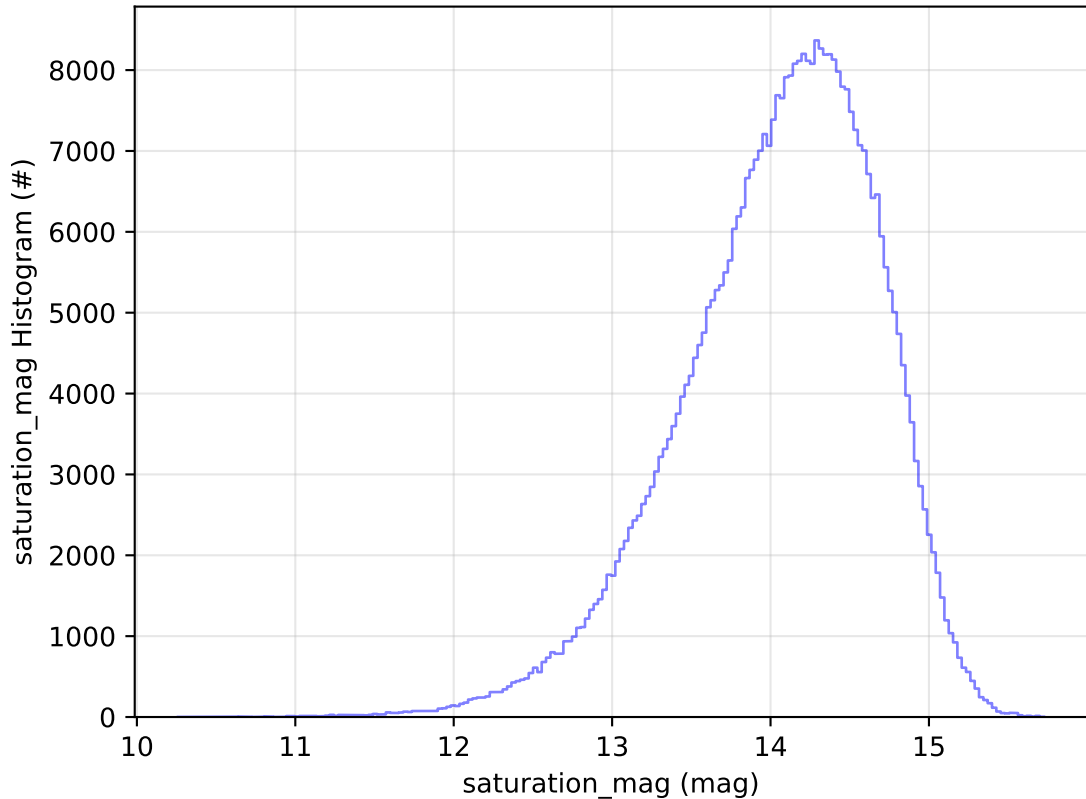
ddf_acor_sf30_lsf40_lsr20_v3.4_10yrs All sky z band: saturation_mag Histogram
