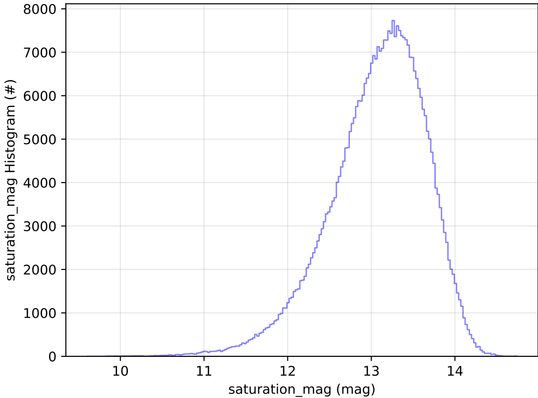
ddf_acor_sf30_lsf40_lsr20_v3.4_10yrs All sky y band: saturation_mag Histogram
