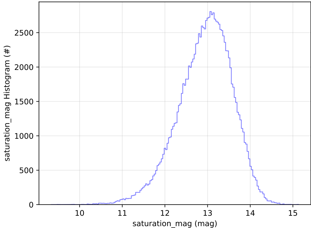
ddf_acor_sf30_lsf40_lsr20_v3.4_10yrs All sky u band: saturation_mag Histogram
