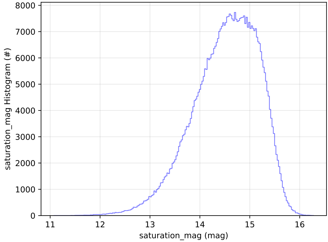
ddf_acor_sf30_lsf40_lsr20_v3.4_10yrs All sky r band: saturation_mag Histogram
