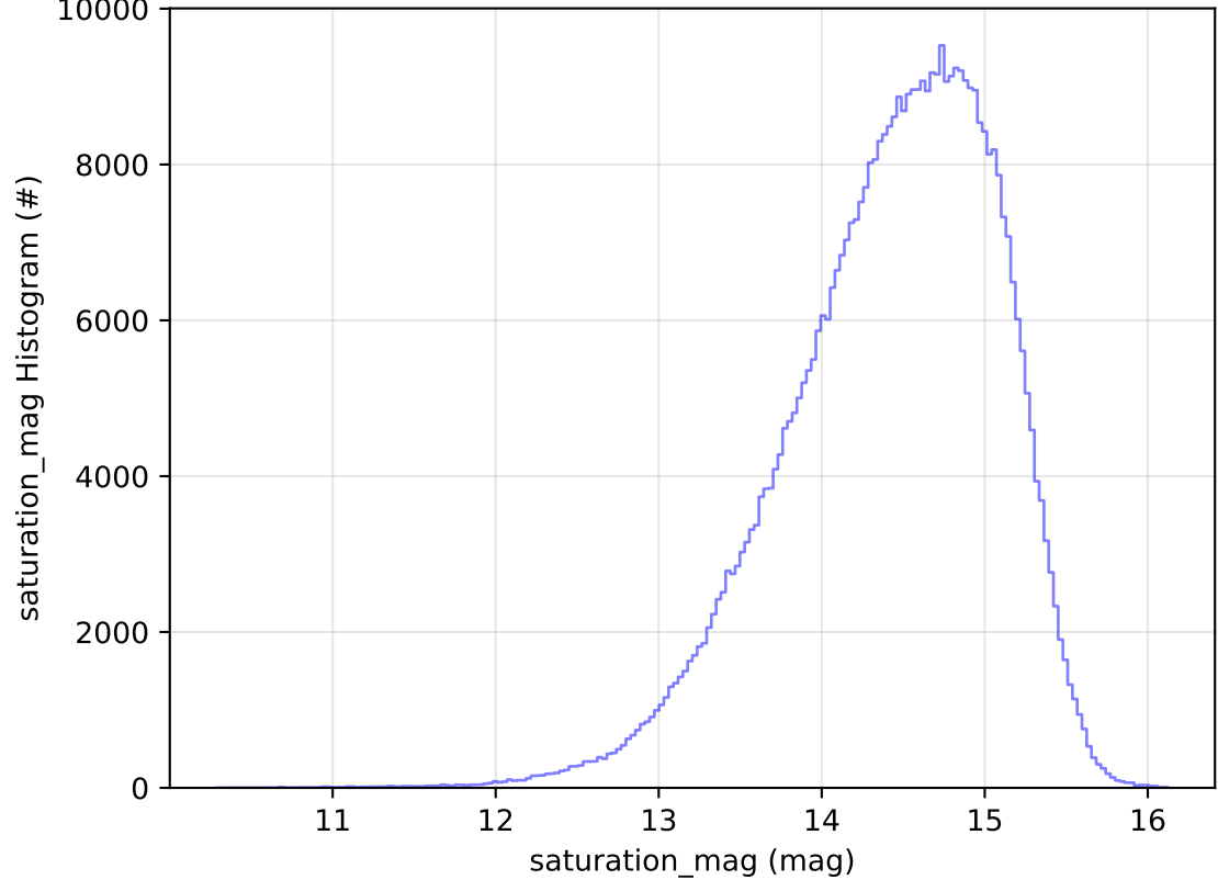
ddf_acor_sf30_lsf40_lsr20_v3.4_10yrs All sky i band: saturation_mag Histogram
