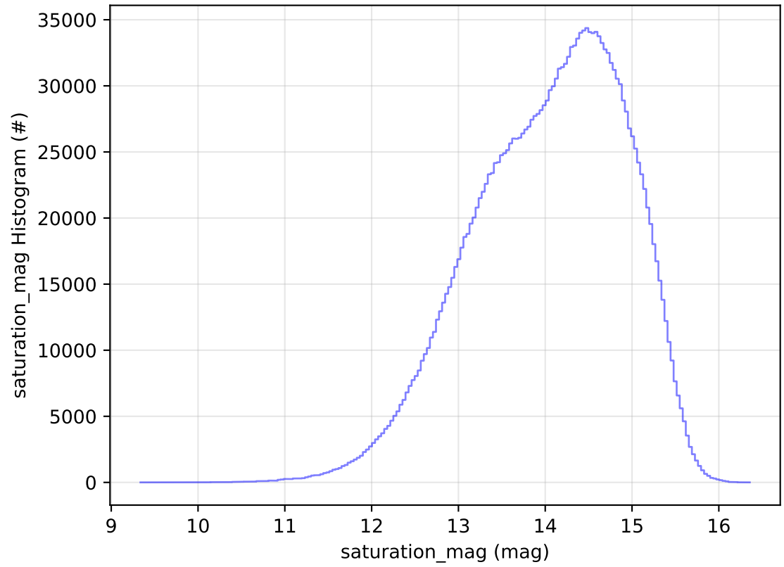
ddf_acor_sf30_lsf40_lsr20_v3.4_10yrs All sky all bands: saturation_mag Histogram
