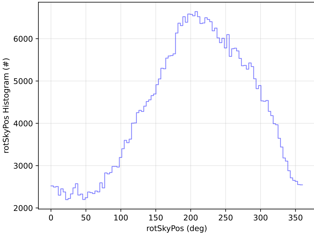
ddf_acor_sf30_lsf40_lsr20_v3.4_10yrs WFD z band: rotSkyPos Histogram
