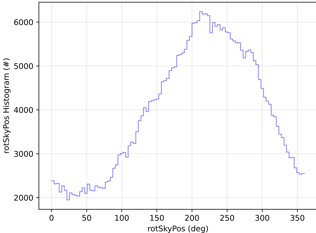
ddf_acor_sf30_lsf40_lsr20_v3.4_10yrs WFD y band: rotSkyPos Histogram
