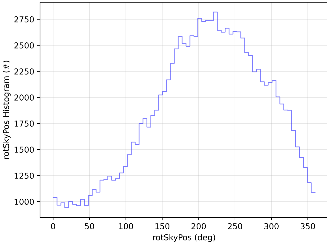
ddf_acor_sf30_lsf40_lsr20_v3.4_10yrs WFD u band: rotSkyPos Histogram
