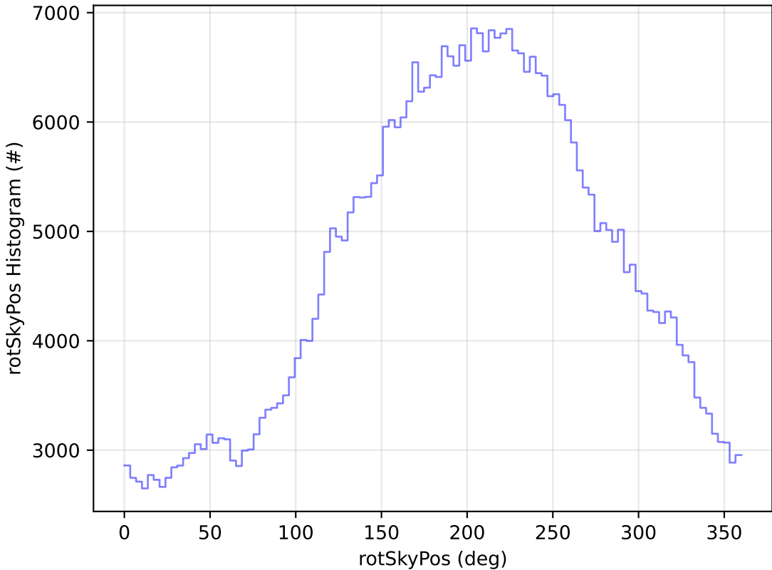
ddf_acor_sf30_lsf40_lsr20_v3.4_10yrs WFD r band: rotSkyPos Histogram
