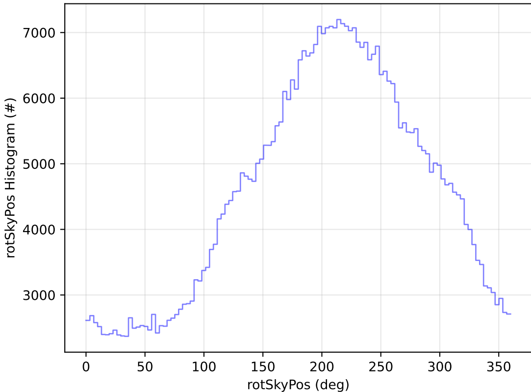
ddf_acor_sf30_lsf40_lsr20_v3.4_10yrs WFD i band: rotSkyPos Histogram
