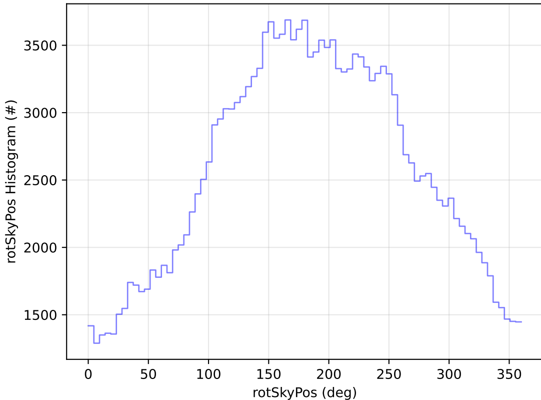
ddf_acor_sf30_lsf40_lsr20_v3.4_10yrs WFD g band: rotSkyPos Histogram
