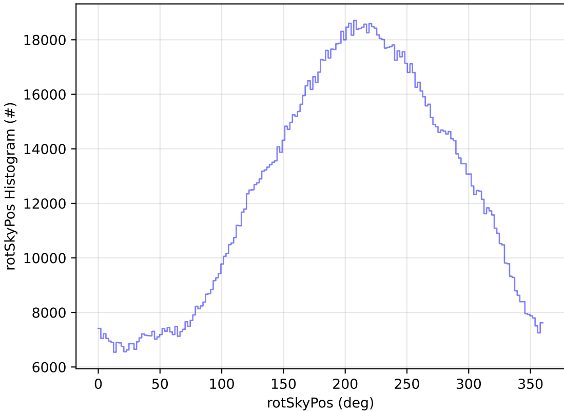
ddf_acor_sf30_lsf40_lsr20_v3.4_10yrs WFD all bands: rotSkyPos Histogram
