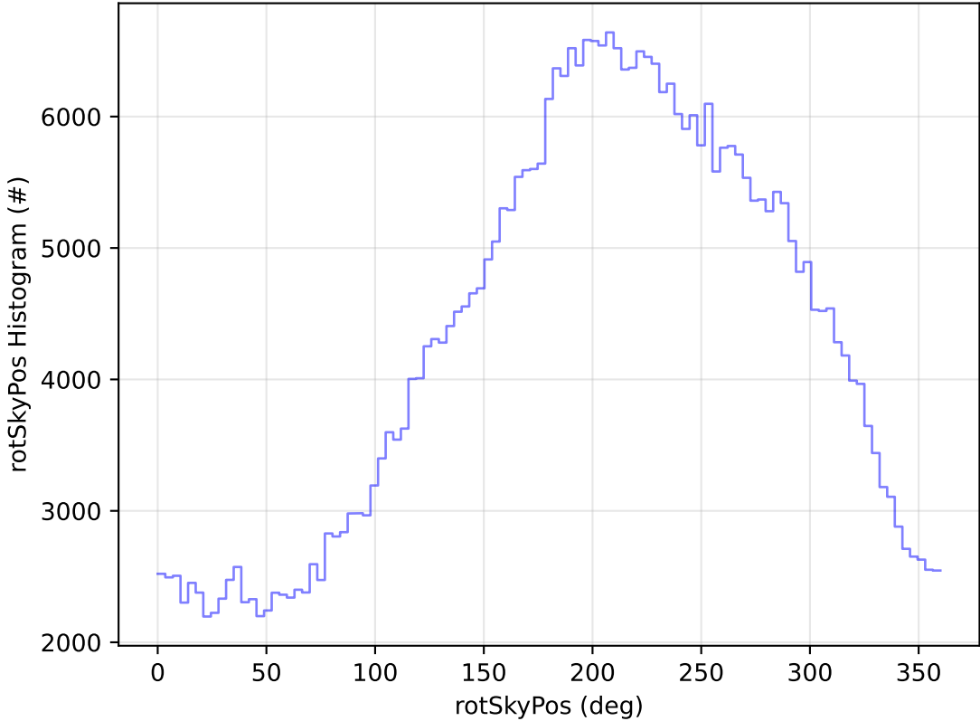
ddf_acor_sf30_lsf40_lsr20_v3.4_10yrs All sky z band: rotSkyPos Histogram
