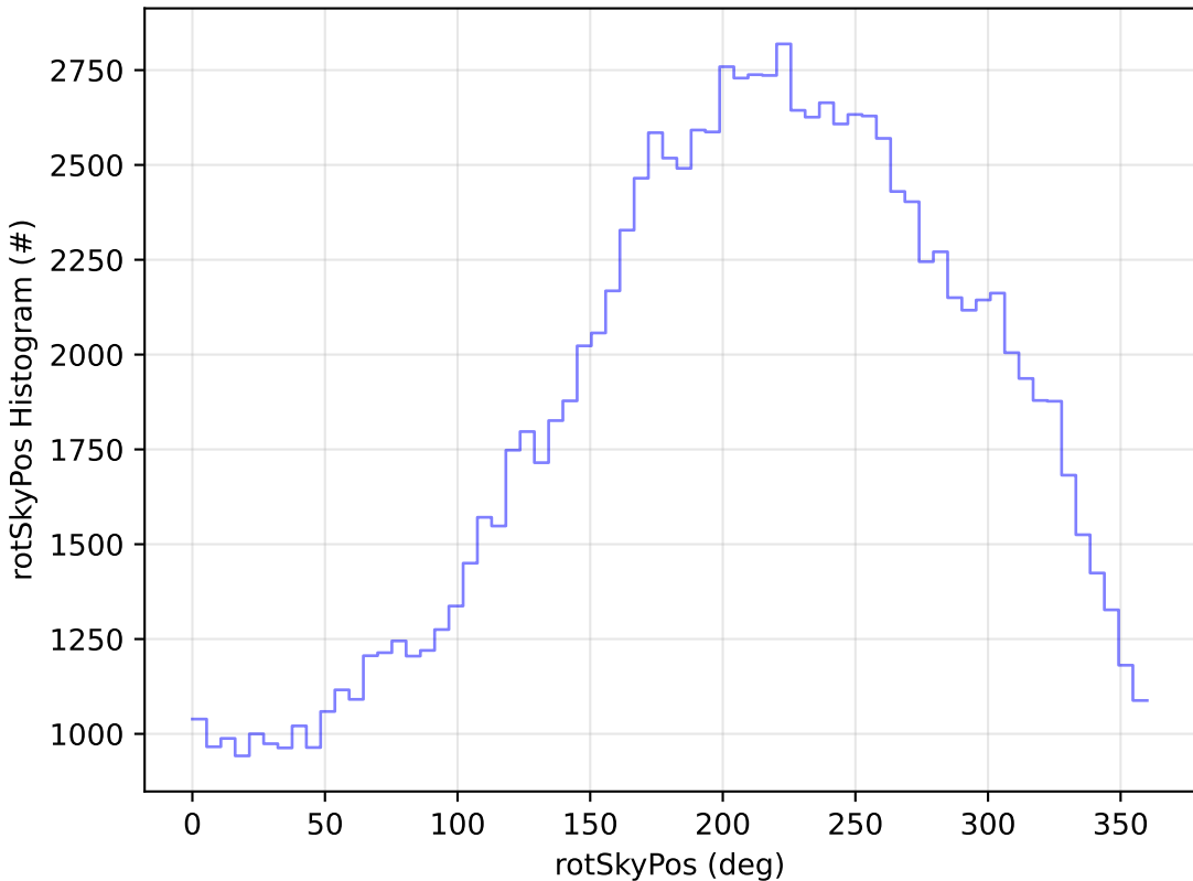
ddf_acor_sf30_lsf40_lsr20_v3.4_10yrs All sky u band: rotSkyPos Histogram
