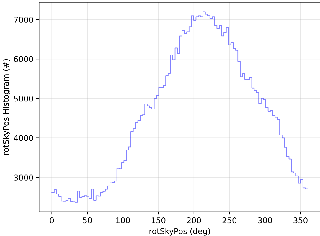
ddf_acor_sf30_lsf40_lsr20_v3.4_10yrs All sky i band: rotSkyPos Histogram
