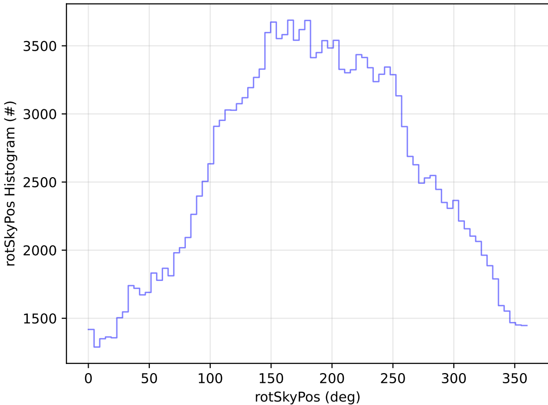
ddf_acor_sf30_lsf40_lsr20_v3.4_10yrs All sky g band: rotSkyPos Histogram
