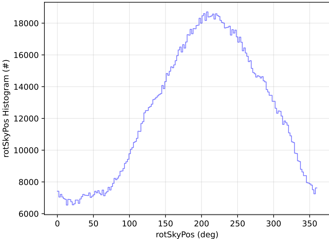
ddf_acor_sf30_lsf40_lsr20_v3.4_10yrs All sky all bands: rotSkyPos Histogram
