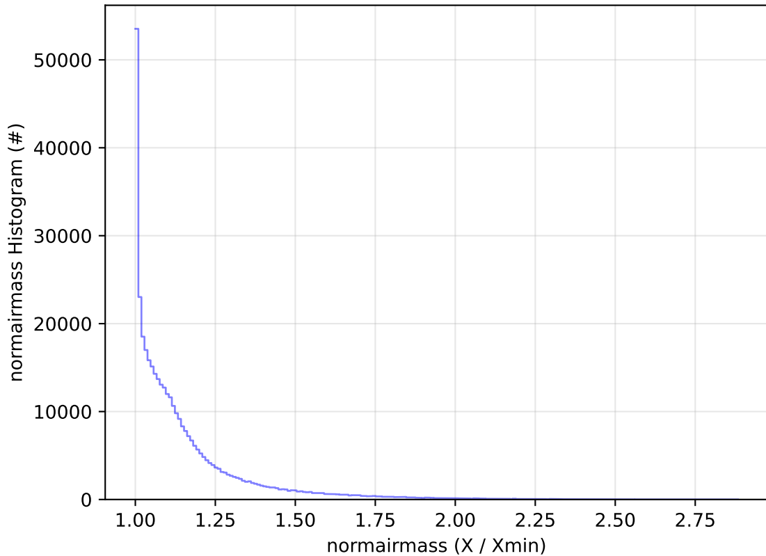
ddf_acor_sf30_lsf40_lsr20_v3.4_10yrs WFD y band: normairmass Histogram
