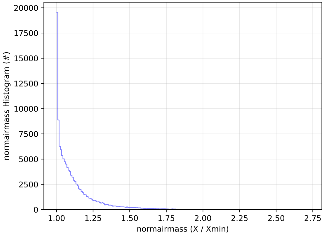
ddf_acor_sf30_lsf40_lsr20_v3.4_10yrs WFD u band: normairmass Histogram
