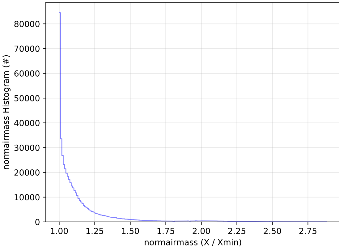
ddf_acor_sf30_lsf40_lsr20_v3.4_10yrs WFD r band: normairmass Histogram
