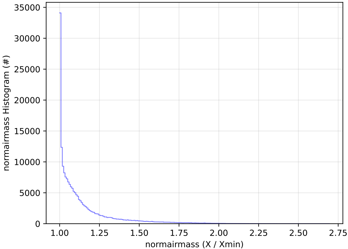
ddf_acor_sf30_lsf40_lsr20_v3.4_10yrs WFD g band: normairmass Histogram
